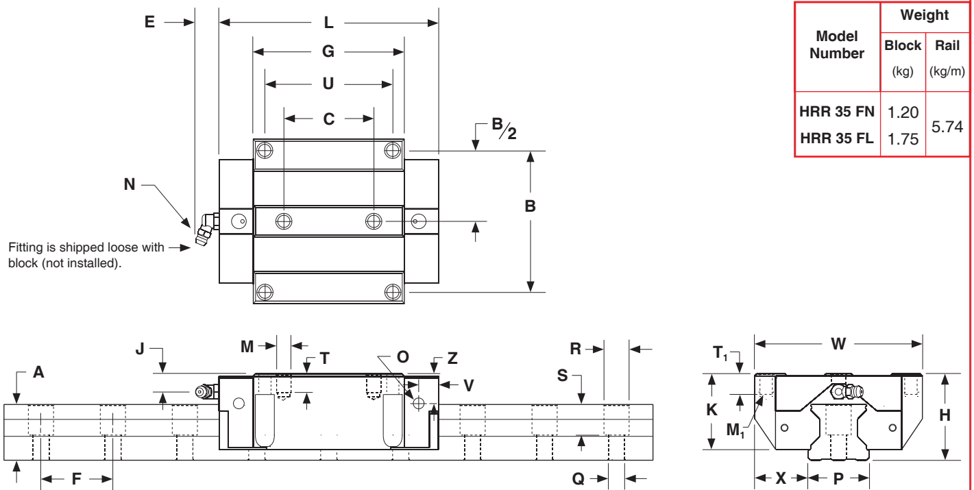
Rail Tapped from Bottom
