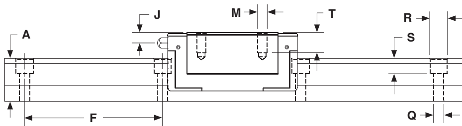
Rail Tapped from Bottom
